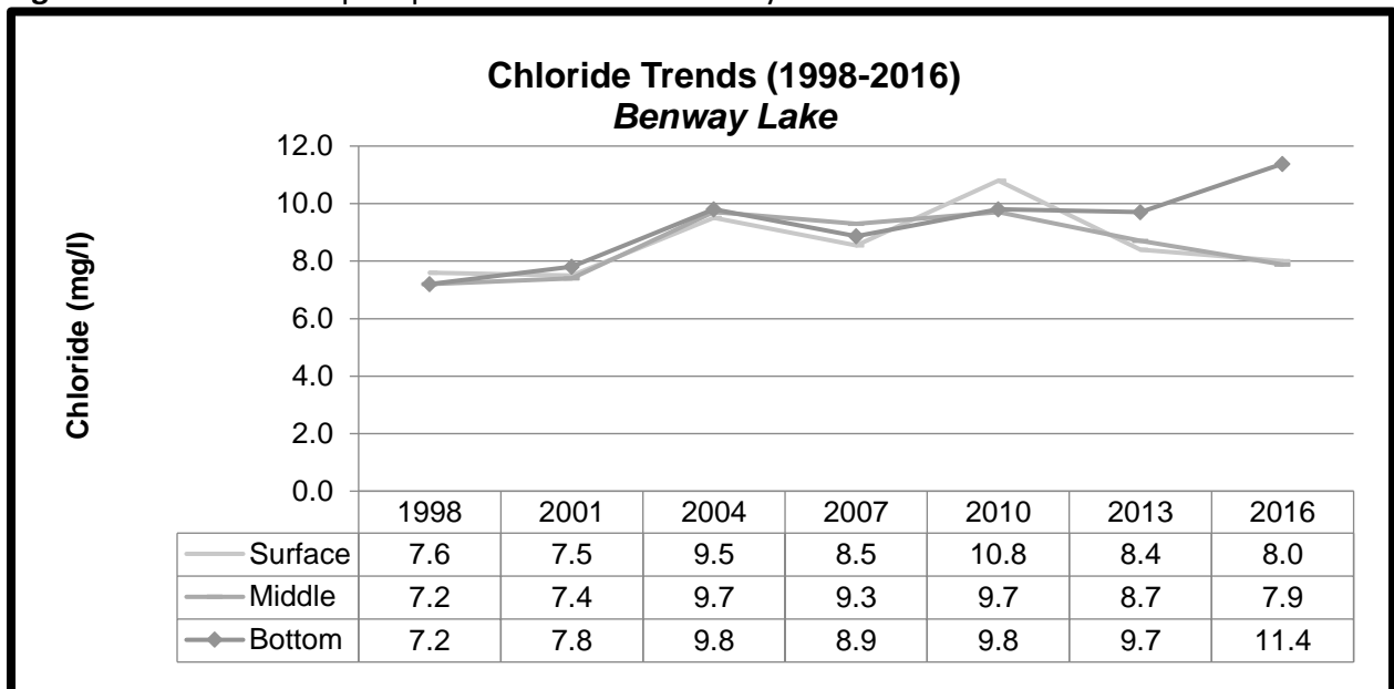
Figure 3. Chart of chloride concentrations in Ben-way Lake.
