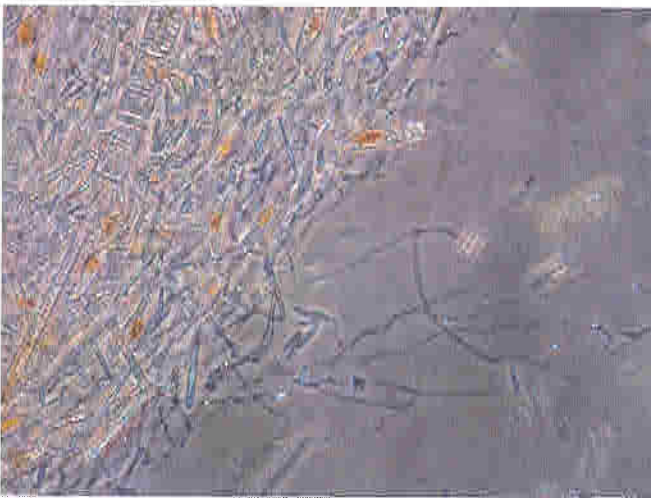
Figure 6. Microscopic image using phase contrast microscopy at 400 × magnification (Bay Harbor Lake sample, March 2006).
