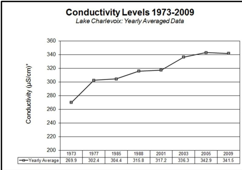
Figure 10: Conductivity levels in Lake Charlevoix from 1973 to 2009
