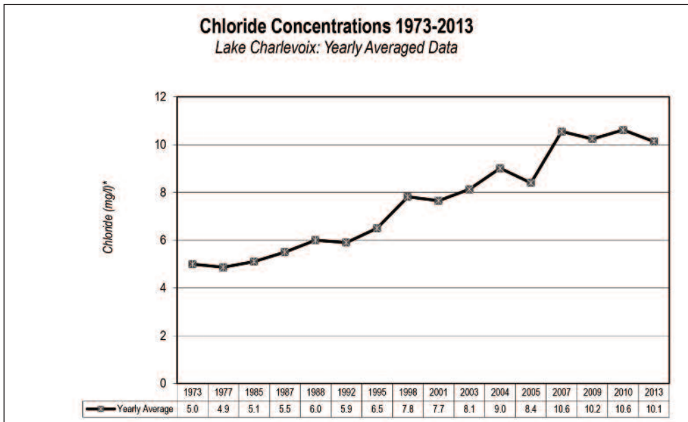
Figure 2 - Chloride Concentrations 1973-2013
