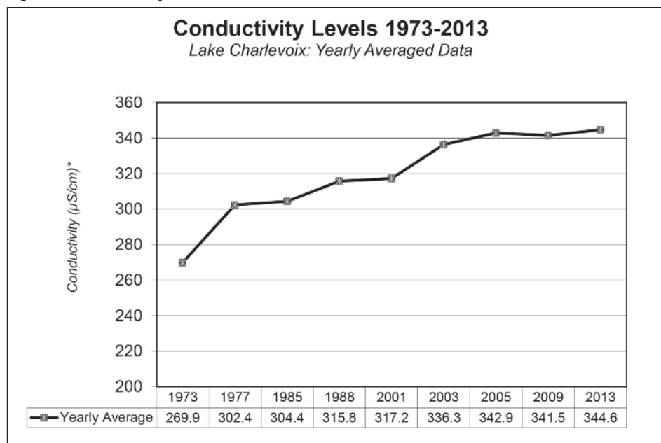
Figure 1 - Conductivity Levels 1973-2013
